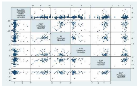
Figure 12: Matrix graph of Model-1
