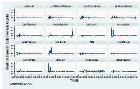
Figure 12(a): Twoway graph of Model-1
